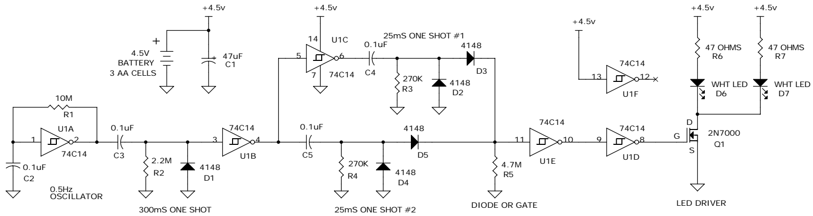
MODEL AIRPLANE WING TIP FLASHER
